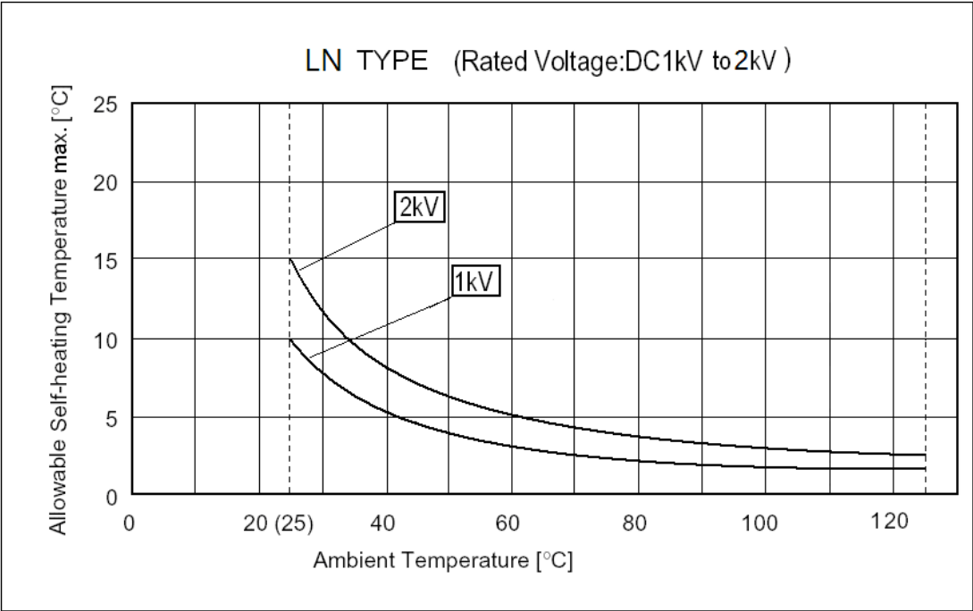
Fig 2 : Dependence of Self-heating Temperature on Ambient Temperature.
